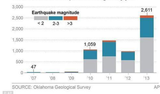
Total number of earthquakes catalogued by year
